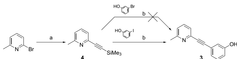
Scheme 1. Reagents and conditions: (a) \text{Me}_3\text{SiC}\equiv\text{CH} , \text{CuI} , \text{PdCl}_2(\text{PPh}_3)_2 , \text{Et}_3\text{N} , rt, 16 h (71%); (b) TBAF, \text{CuI} , \text{PdCl}_2(\text{PPh}_3)_2 , \text{Et}_3\text{N} , DMF, 70 °C, 16 h (67%).
