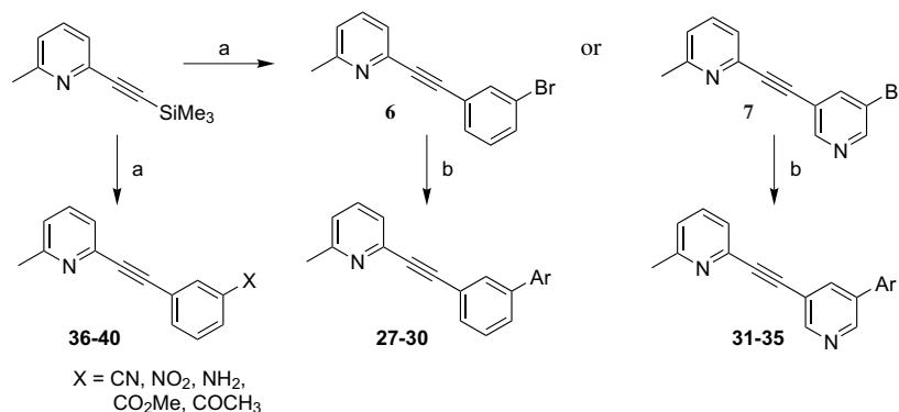
Scheme 3. Reagents and conditions: (a) aryl or heteroaryl bromide, CuI, PdCl 2 (PPh 3 ) 2 , Et 3 N, Bu 4 NF, DMF, 70 °C; (b) aryltrialkylstannane, Pd(PPh 3 ) 4 , toluene, reflux.
