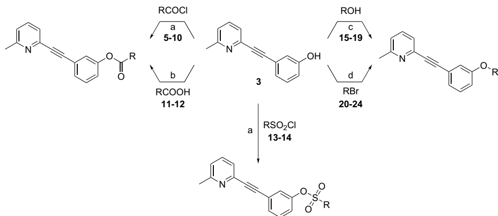
Scheme 2. Reagents and conditions: (a) \text{Et}_3\text{N} , THF, rt, 3–16 h (70–97%); (b) DCC, DMAP, THF, rt, 16 h (89–93%); (c) \text{PPh}_3 , DEAD, THF, rt, 3 h (73–91%); (d) \text{NaH} , THF or DMF, rt, 16 h (65–97%).
